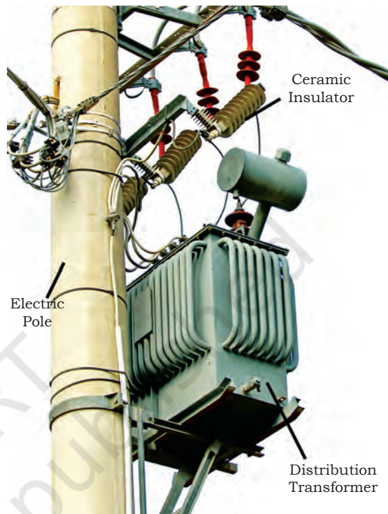
Fig.1.3: Distribution of electric power for residential use
