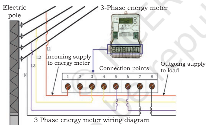
Fig. 10.9: Circuit connection of a three-phase energy meter
