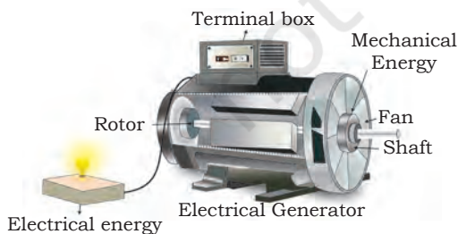
Fig.1.10: An electrical generator converts mechanical energy into electrical energy
