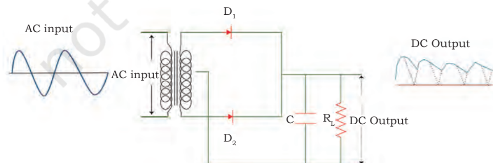
Fig. 7.21: Full wave rectifier with capacitor filter
