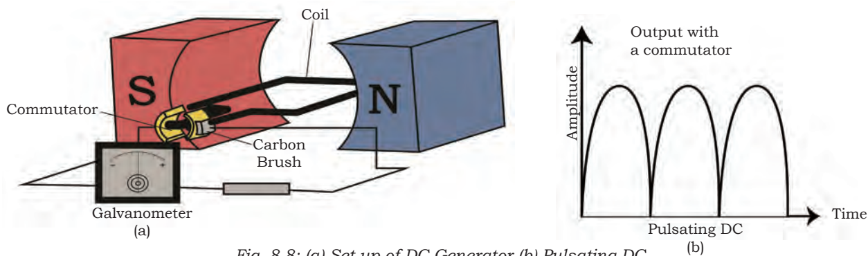
Fig. 8.8: (a) Set up of DC Generator (b) Pulsating DC
