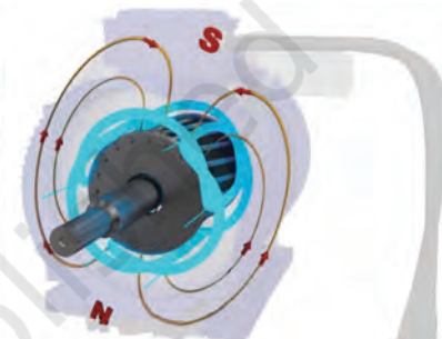
Fig. 8.24: Rotating magnetic field in the squirrel cage induction motor
