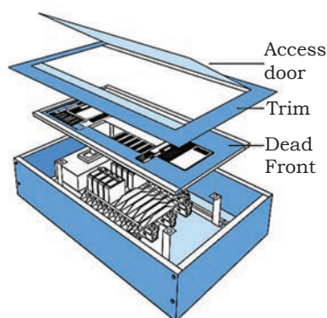
Fig. 5.15: Dead front and trim in the panel board
