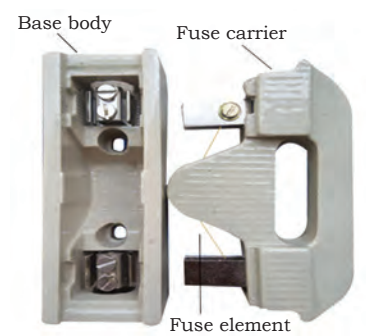
Fig. 3.11: The different parts of a fuse
