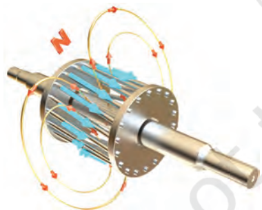
Fig. 8.25: EMF is induced in the rotor conductor
