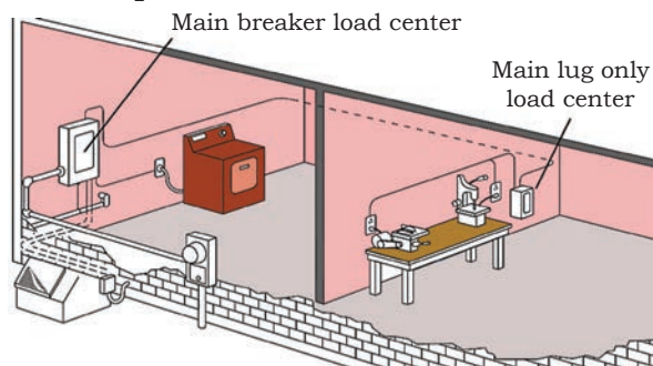
Fig. 4.15: Installation of a main breaker load centre and main lug only load centre
