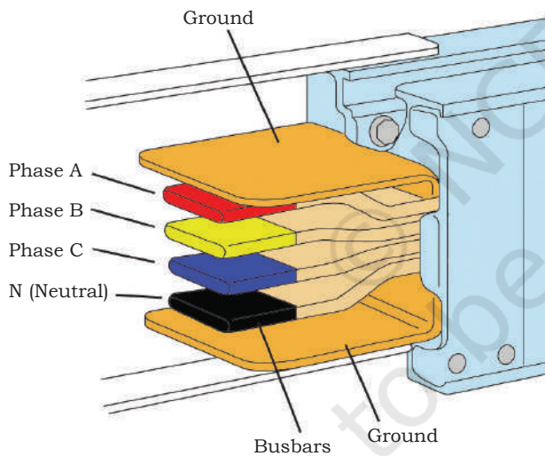
Fig. 2.15: Busbar representing phases in a busway
