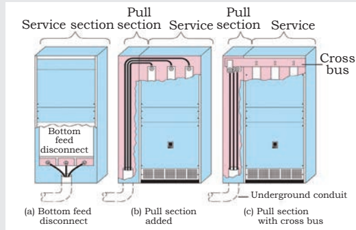
Fig. (a.) Different feeding methods in a switchboard
