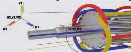
Fig. e: Connect terminal 2 of coil 'U', coil 'V', coil 'W' together
