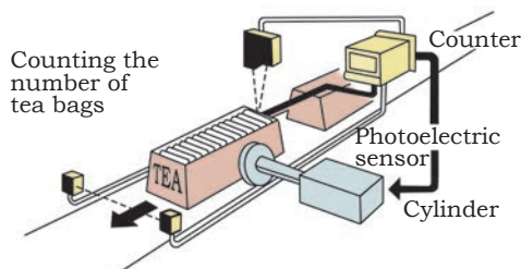
Fig. 9.5: PLC counting the number of tea bags
