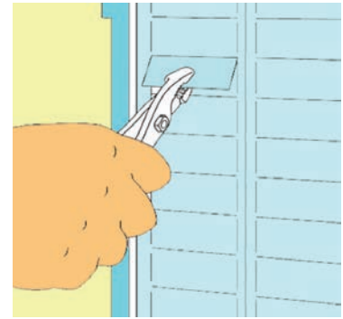
Fig. 4.12: Trim assembly
