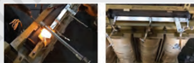
Fig. k: Making of coil terminals connection for the secondary winding. The coil terminal is connected in such a way that it forms a star configuration.
