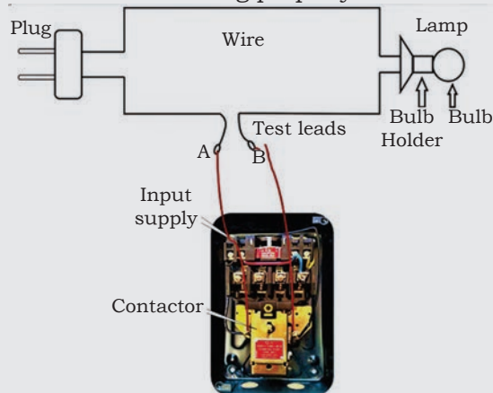
Fig. b: Test circuit for testing the contactor
