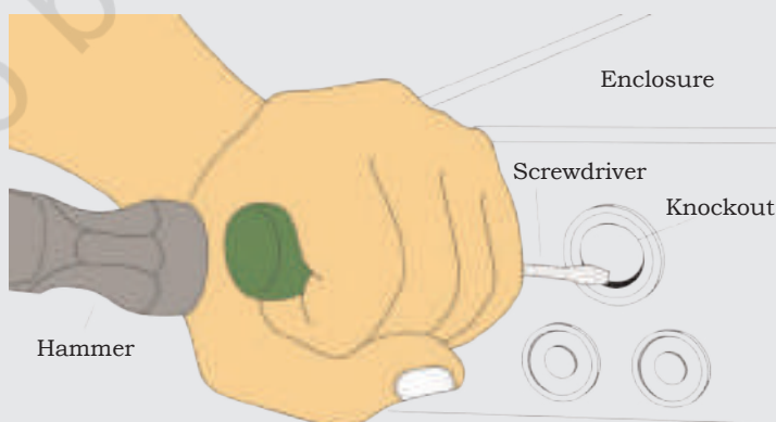
Fig. b: Removing knockouts
