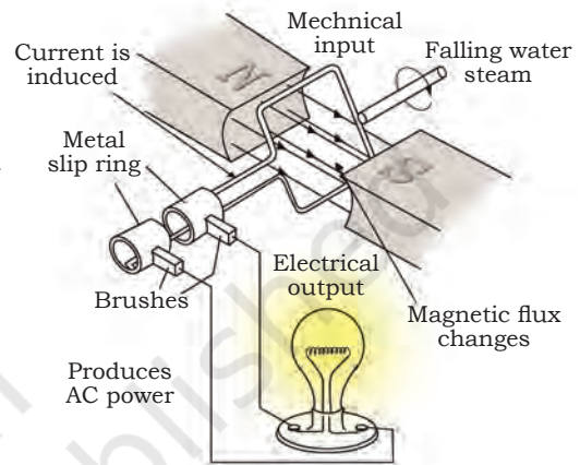
Fig.1.12: The basic principle of an AC generator
