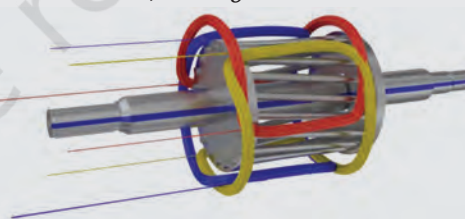
Fig. d: Blue coil represents 'U' coil, red coil represents 'V' coil, yellow coil represents 'W' coil
