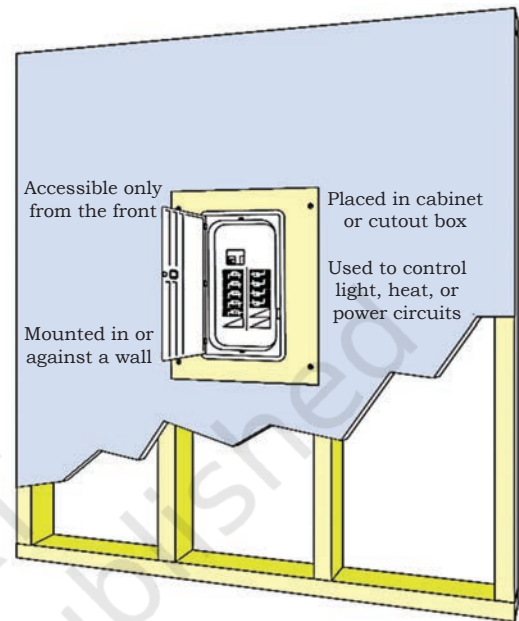
Fig. 4.5: Load centre mounted on a wall
