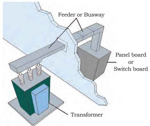
Fig. 1.40: Service entrance
